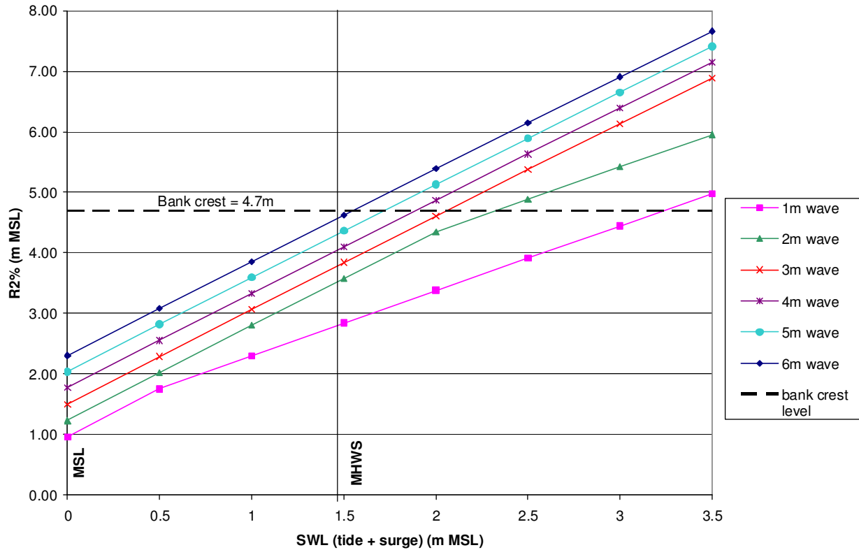
Figure 3 Run-up elevations exceeded by 2% of waves according to still water level and significant wave height
